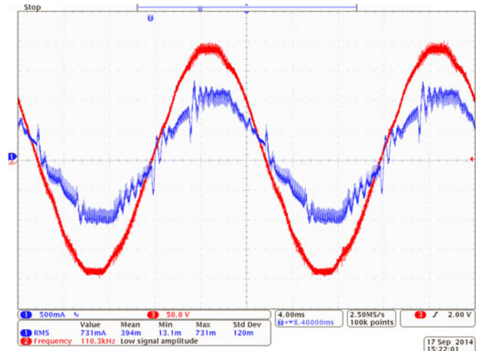
Fig. 16. Experimental results. Phase grid voltage (red trace, 50 V/div) and injected current (blue trace, 0.5 A/div, THD = 11%) in the case of the base SVM.
