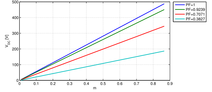
Fig. 7. Relation between the modulation index and the V_{DC} of the PV module.
