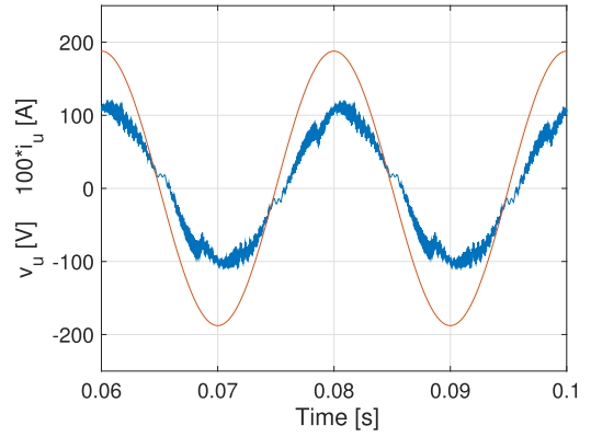
Fig. 10. Simulation results. Phase grid voltage and injected current (THD = 8.2%) in the case of the adopted SVM for the CSI7 topology without overlap compensation.
