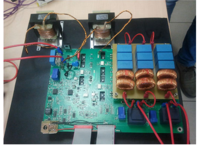
Fig. 15. Power board of the CSI7 laboratory prototype.
