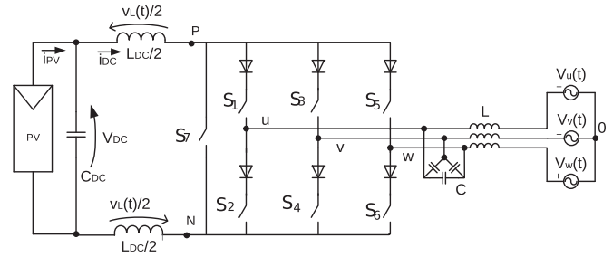
Fig. 1. Three-phase CSI7 topology.
