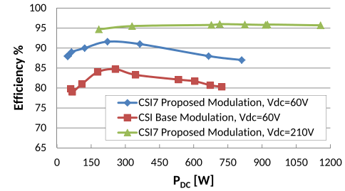
Fig. 23. Experimental results. Efficiency comparison between the CSI7 solution and the traditional CSI solution.
