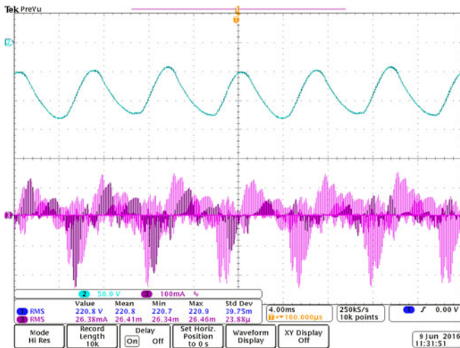
Fig. 21. Experimental results. Ground voltage (50 V/div) and ground leakage current (100 mA/div) in the case of the CSI7 solution.
