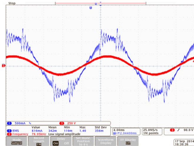
Fig. 18. Experimental results. Phase grid voltage (red trace, 250 V/div) and injected current (blue trace, 0.5 A/div, THD = 11.5%) in the case of the adopted SVM for the CSI7 topology without the inversion sequence.
