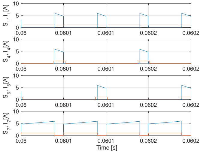
Fig. 13. First sextant operation: switching sequence and device currents of S_1 , S_4 , S_6 , and S_7 .
