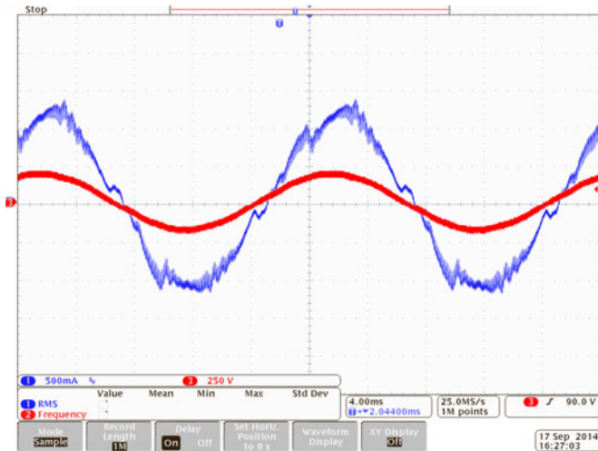
Fig. 17. Experimental results. Phase grid voltage (red trace, 250 V/div) and injected current (blue trace, 0.5 A/div, THD = 8.9%) in the case of the adopted SVM for the CSI7 topology without overlap compensation.
