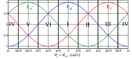
Fig. 3. Grid phase voltages with sector numbers of the SV current in the case of unity power factor.
