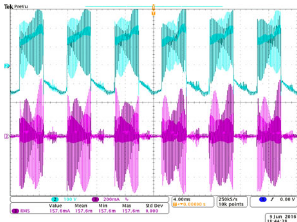
Fig. 22. Experimental results. Ground voltage (100 V/div) and ground leakage current (200 mA/div) in the case of the base SVM for the traditional CSI topology.
