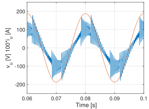
Fig. 11. Simulation results. Phase grid voltage and injected current (THD = 25%) in the case of the adopted SVM for the CSI7 topology without the inversion sequence.
