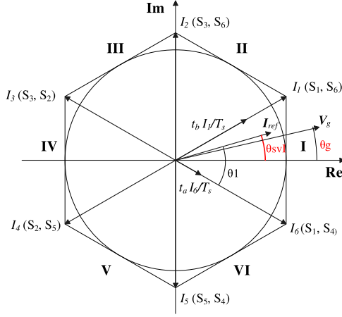
Fig. 2. SV representation.
