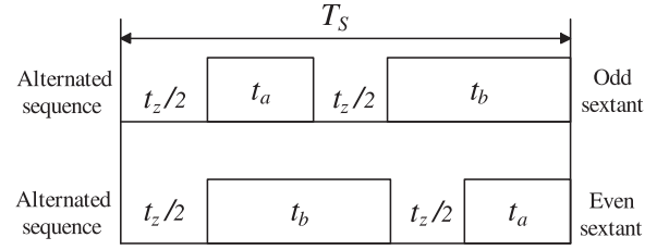
Fig. 5. Alternated sequence; details of commutation sequence for even and odd sextants to avoid glitch generation.
