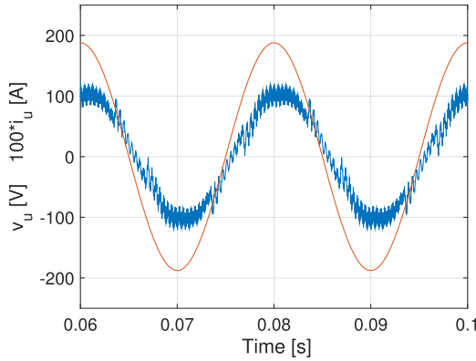
Fig. 9. Simulation results. Phase grid voltage and injected current (THD = 11.88%) in the case of the base PWM for the traditional CSI topology.
