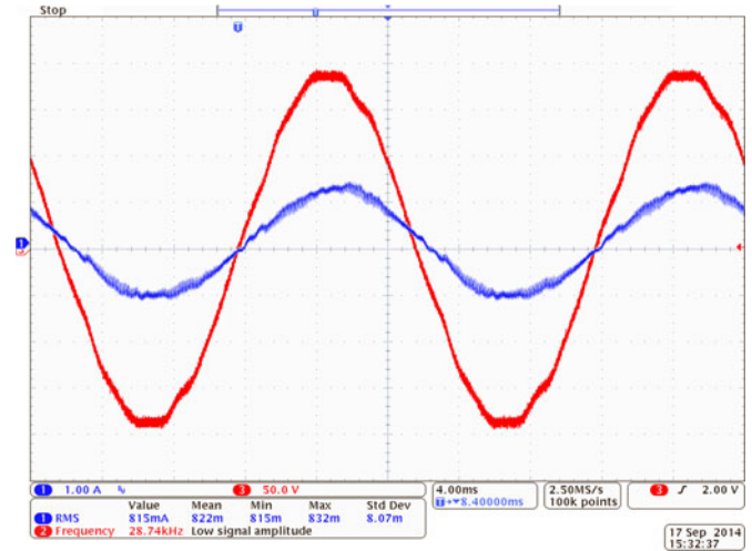
Fig. 19. Experimental results. Phase grid voltage (red trace, 50 V/div) and injected current (blue trace, 1 A/div, THD = 4.5%) in the case of the complete adopted SVM for the CSI7 topology.
