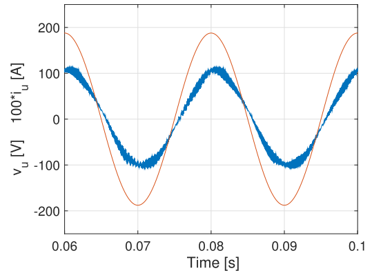
Fig. 12. Simulation results. Phase grid voltage and injected current (THD = 4.4%) in the case of the adopted SVM for the CSI7 topology.
