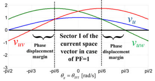
Fig. 4. Power factor operation range to guarantee a positive voltage across S_7 during sector I.
